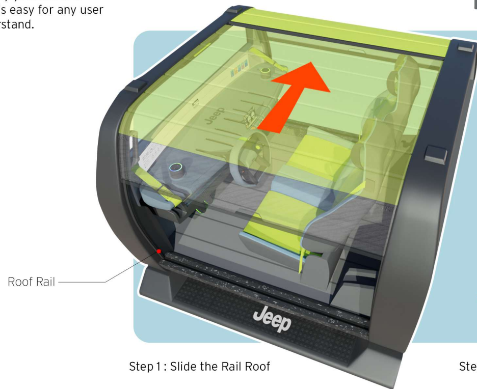
Sliding-Type Rail roof System
